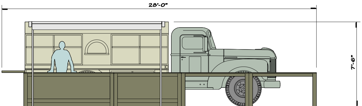
ELEVATION OF OPENED TRUCK w/ TABLES
